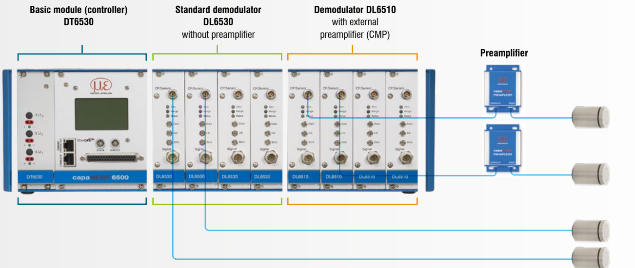
Max. 8 sensors on one DT6500
