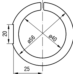
MA 2405-40 for sensor IFS2405-6
