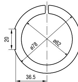
MA 2405-62 for sensors IFS2405-28 / -30
