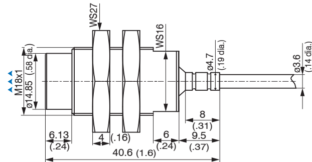
ES-U6-C-CAx, dimensions in mm (inches, rounded off)
