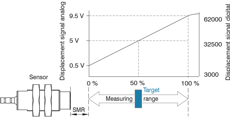
Start of measuring range (SMR), the shortest distance between the front surface of the sensor and the target.
