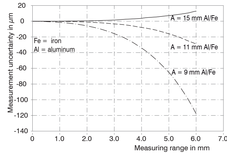
Measurement uncertainty depending on distance A and target material
